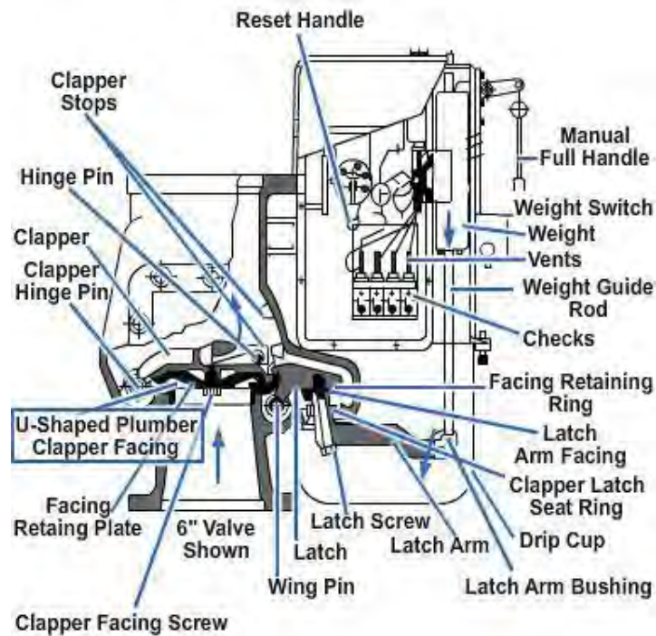
Figure 4-9 – Deluge valve.
